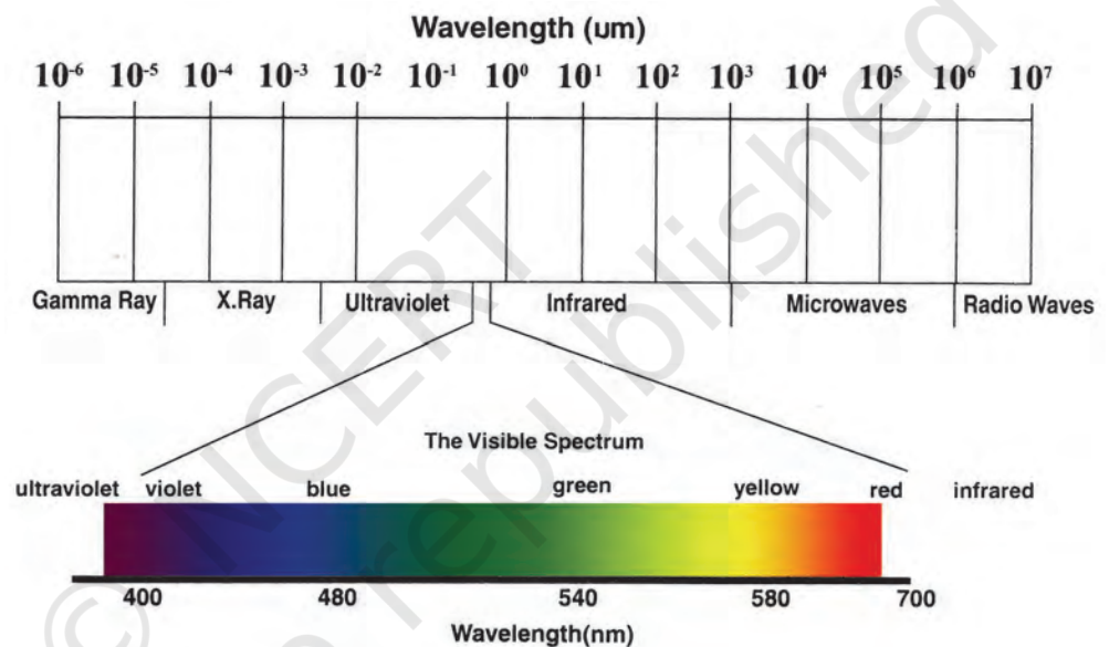
Figure 6.3 Electromagnetic Spectrum
